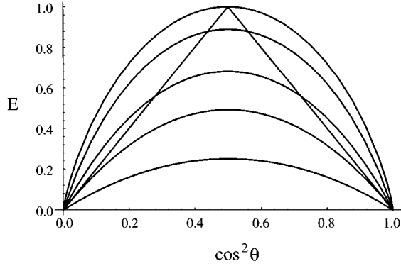
FIG. 1. Yield of maximally entangled output states from partly entangled input states ( \cos\theta|\downarrow - \sin\theta|\uparrow ), as a function of \cos^2\theta . Highest curve is entropy of entanglement of input state, equal to the asymptotic yield of the Schmidt projection method. Successively lower smooth curves give yields of Schmidt projection applied to n = 32, 8, 4, and 2 input pairs. The inverted-V-shaped curve gives yield by the Procrustean method applied to one input pair.
